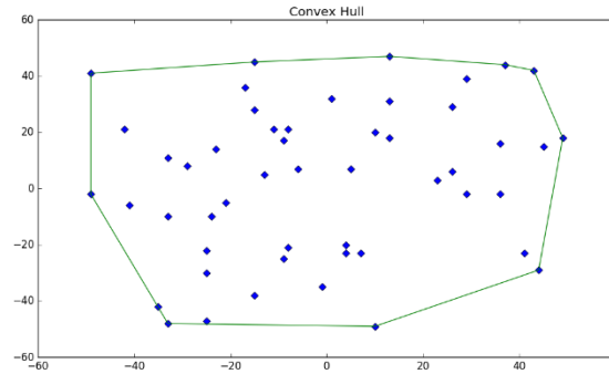
Figure 10: convex hull
