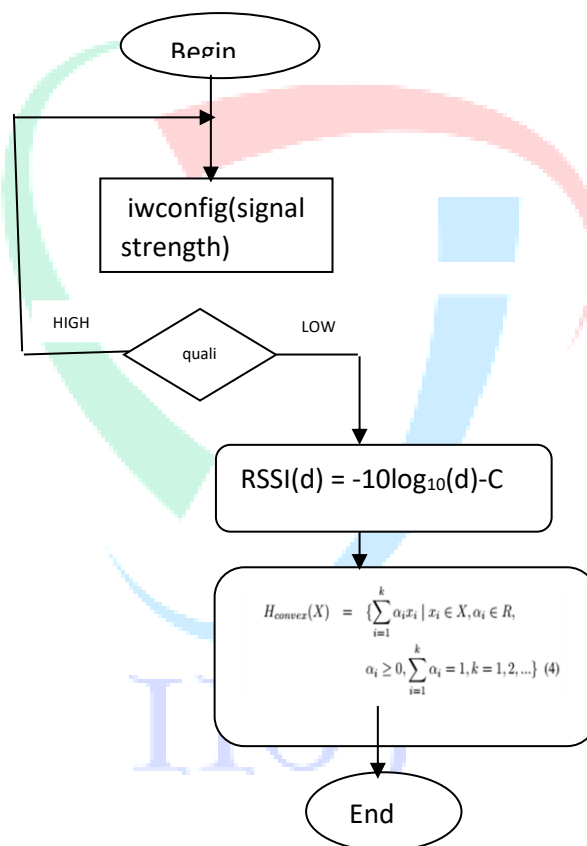
Figure 6: Algorithm representation
