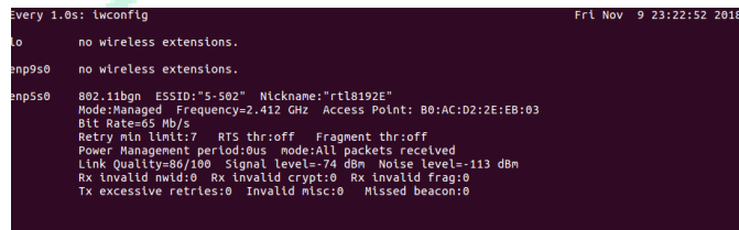
Figure 8: iwconfig command
