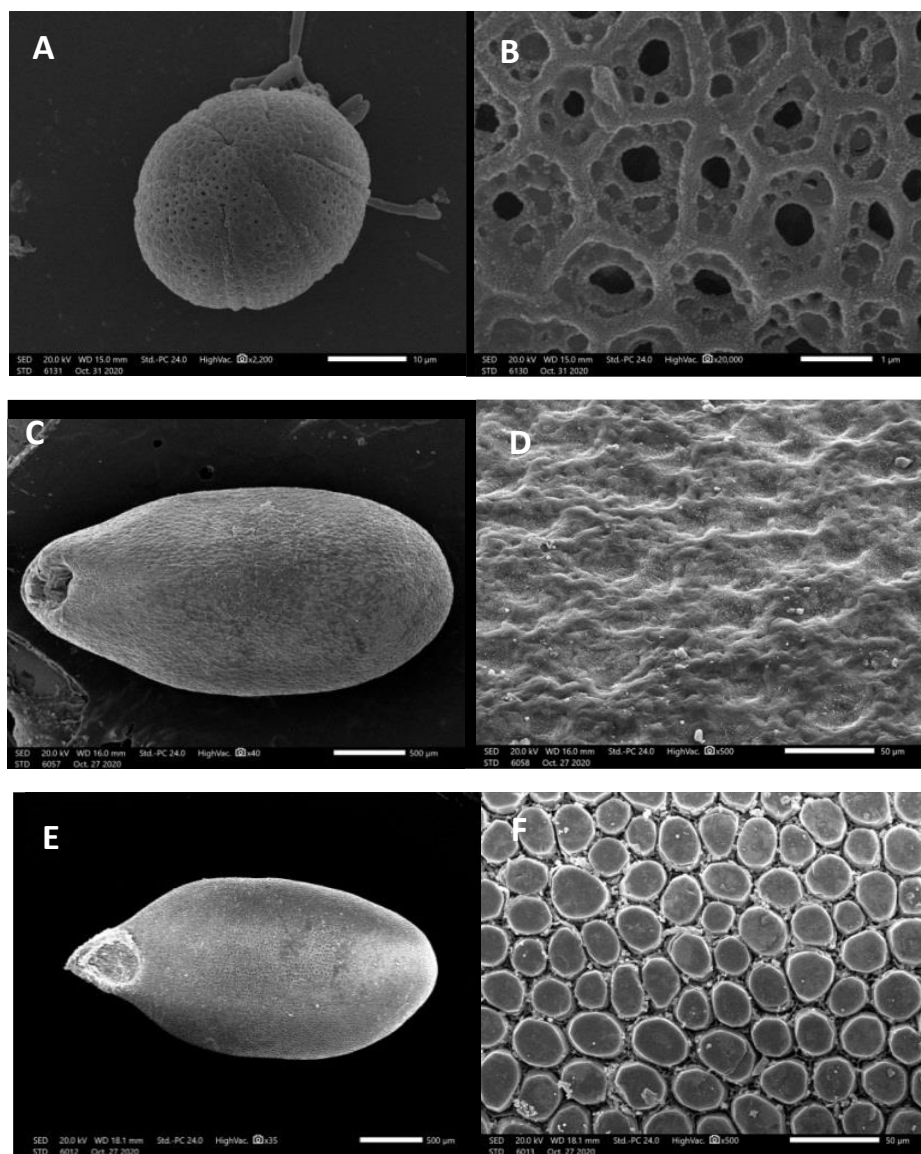
Figure3: Scanning electron micrographs of Salviaviridis : A-Pollen grain shape; B- Pollen grain ornamentation; C- Nutlet shape; D- Nutlet surface ornamentation; E-Seed shape; F- Seed ornamentation.
